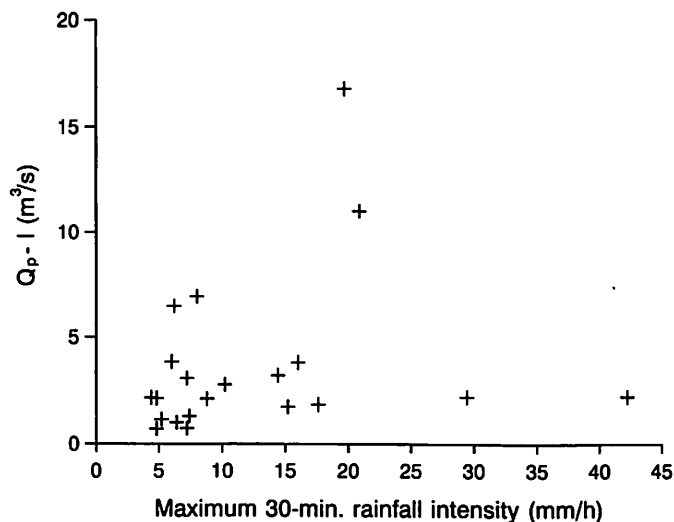
Fig. 10. Peak flow ( Q_p ) above antecedent flow ( I ) versus maximum 30-min rainfall intensity.
