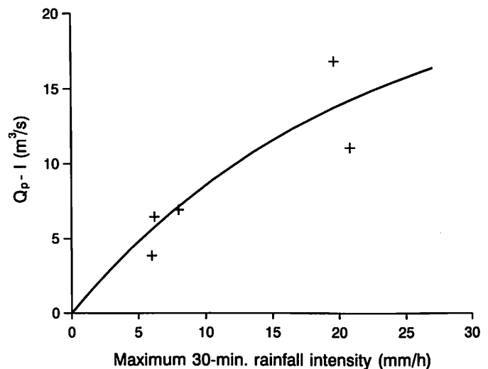
Fig. 13. Peak flow ( Q_p ) above antecedent flow ( I ) versus 30-min rainfall intensity ( Q_p > 5 ).
