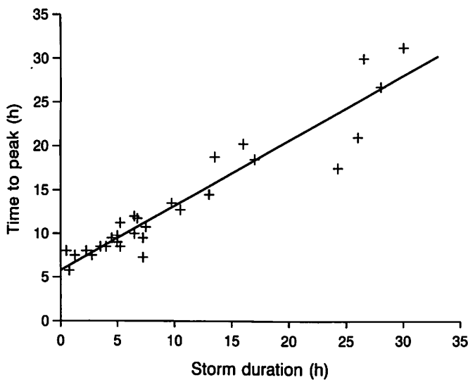
Fig. 5. Time to peak flow versus rainfall (storm) duration.
