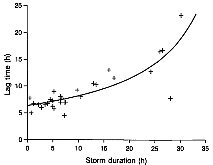
Fig. 4. Lag time versus rainfall (storm) duration.
