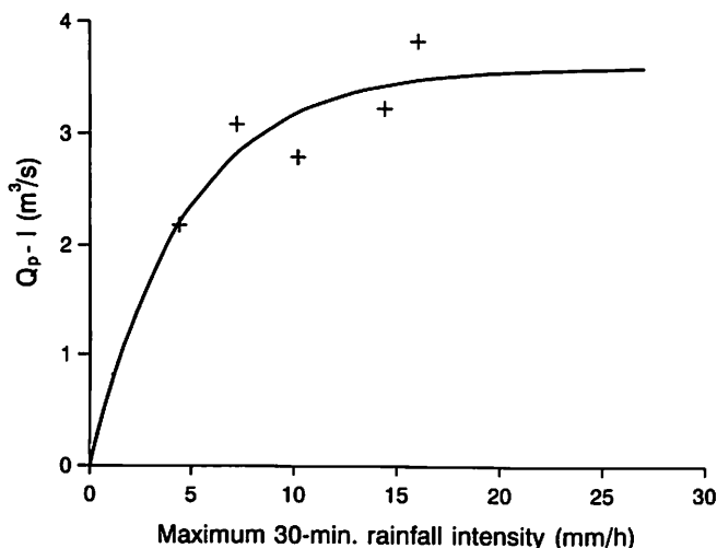
Fig. 12. Peak flow ( Q_p ) above antecedent flow ( I ) versus 30-min rainfall intensity ( 5 > Q_p > 3 ).
