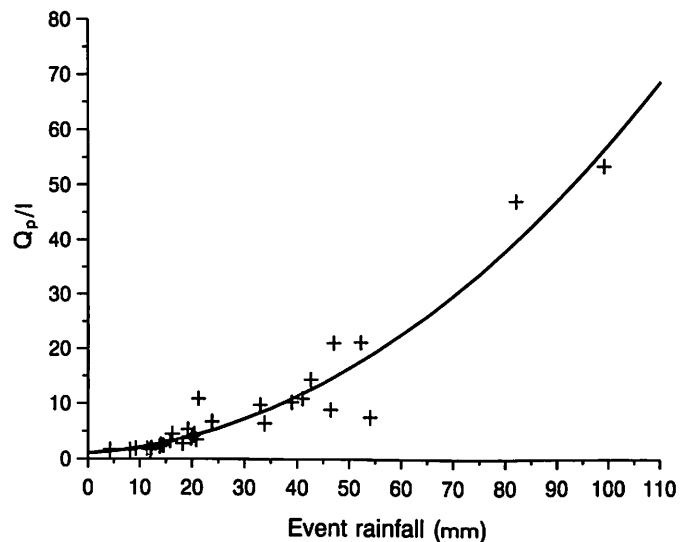
Fig. 7. Peak flow ( Q ) to antecedent flow ( I ) ratio versus event rainfall volume.
