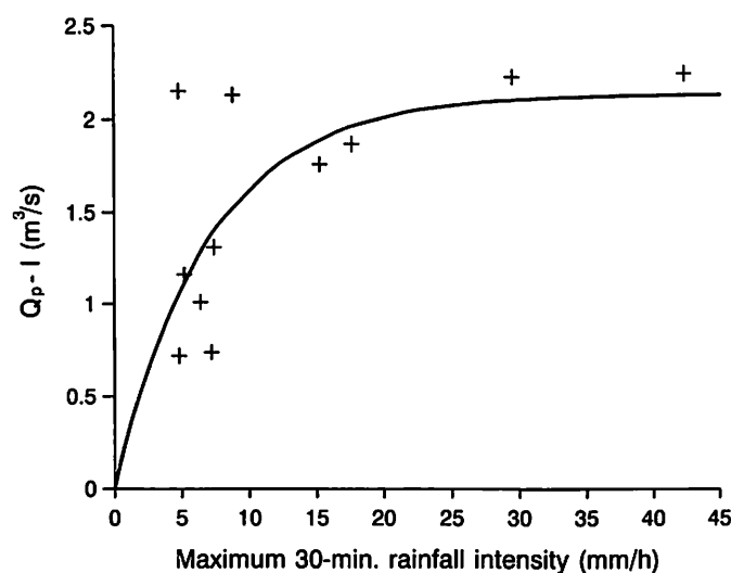
Fig. 11. Peak flow ( Q_p ) above antecedent flow ( I ) versus 30-min rainfall intensity ( 3 > Q_p > 1 ).
