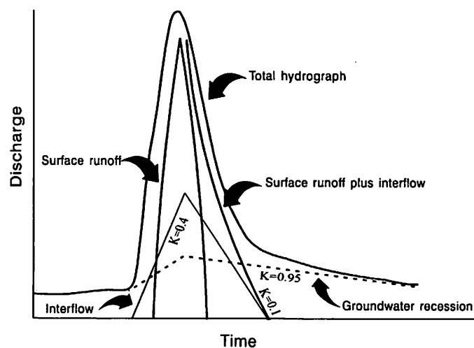
Fig. 3. Hydrograph properties.
