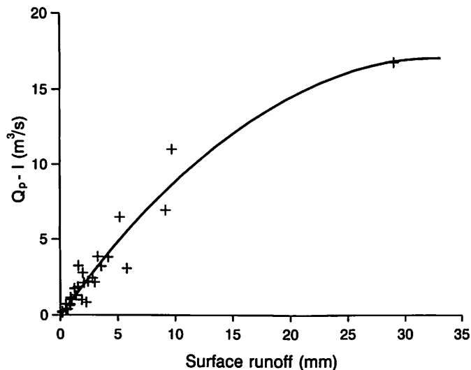
Fig. 8. Peak flow ( Q_p ) above antecedent flow ( I ) versus surface runoff.
