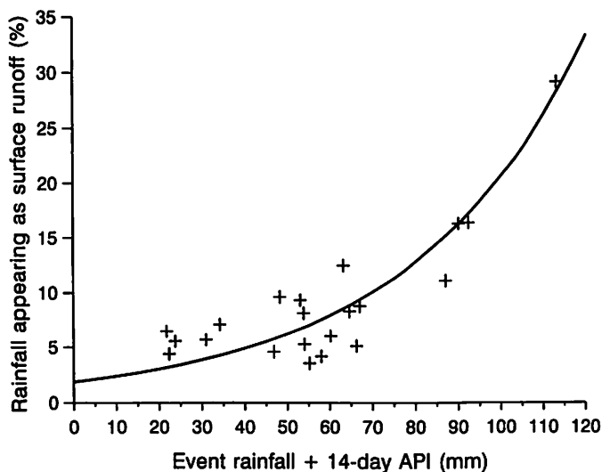
Fig. 9. Rainfall appearing as surface runoff versus cumulative event rainfall and 14-day Antecedent Precipitation Index.
