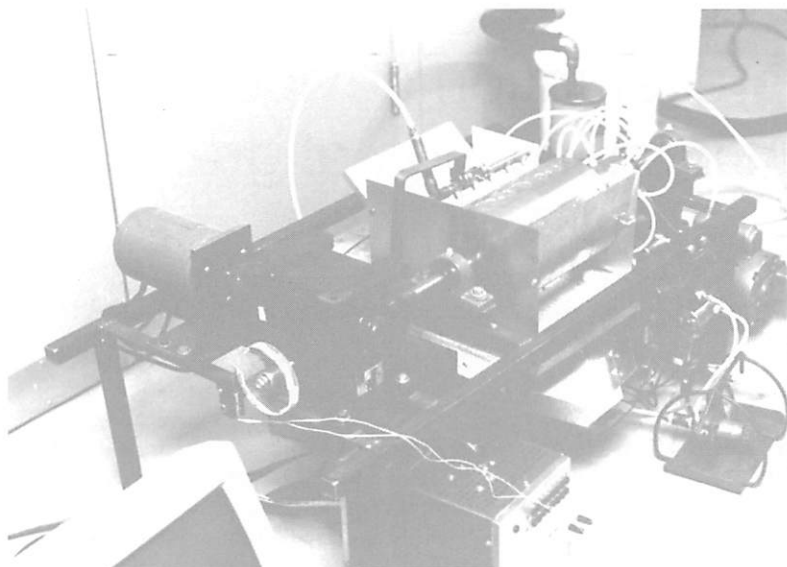
Fig. 1. Assembled components of a seed singulation and presentation device.
