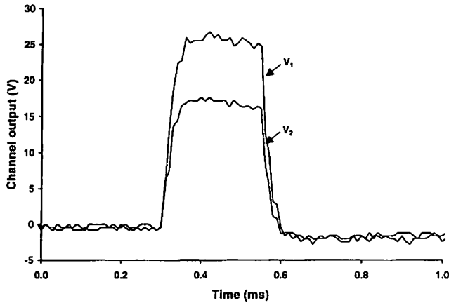
Fig. 3. Voltage waveforms from the monitoring circuitry. V_1 is the voltage output from the TENS device. V_2 is the voltage drop across the resistor and represents the current in the circuit.
