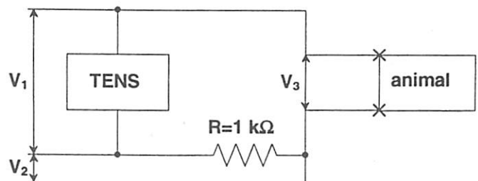
Fig. 2. Electrical configuration for monitoring the performance of the TENS device.
